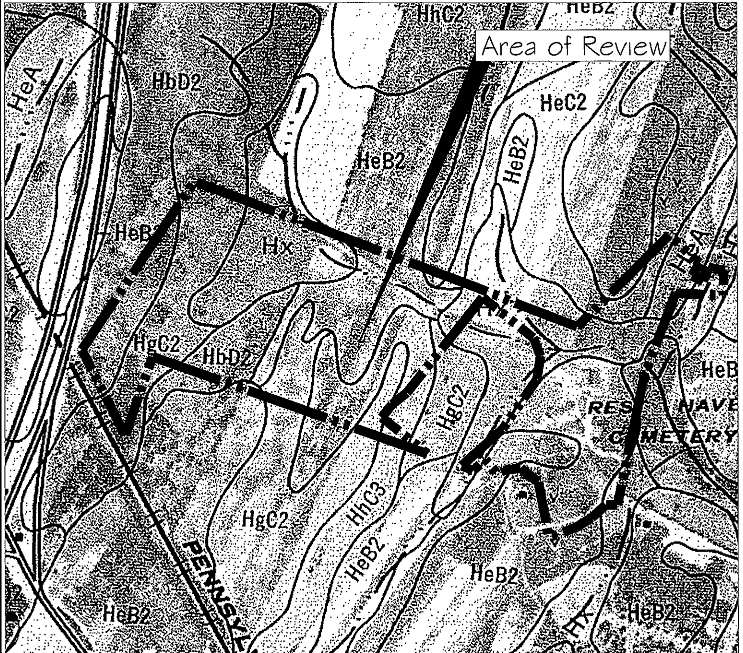
Figure 4: Washington County, Maryland Soil Survey
